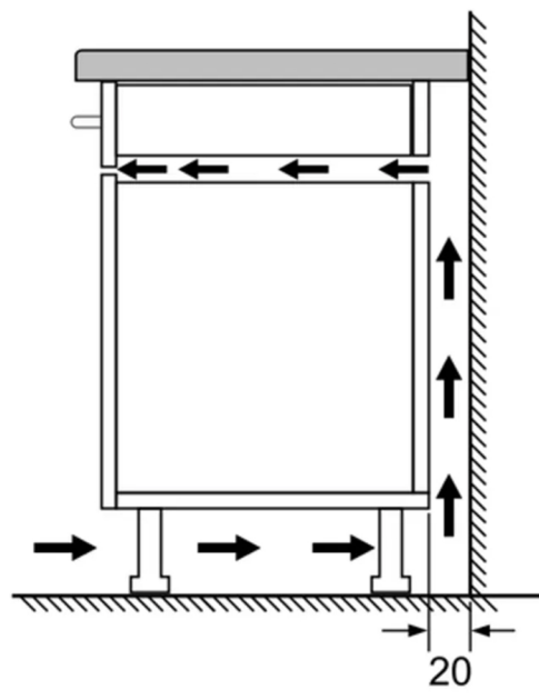
measurements in mm
