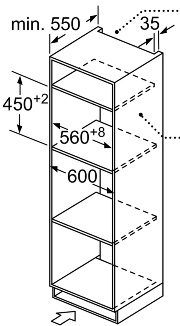
Ventilation space in the base min. 50 cm 2
