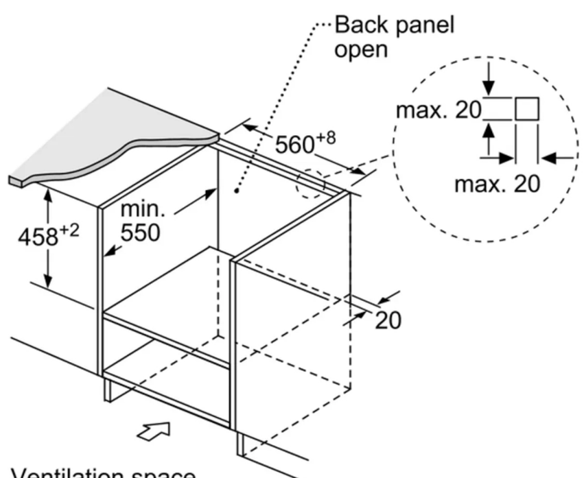
Ventilation space in the base min. 50 cm 2
